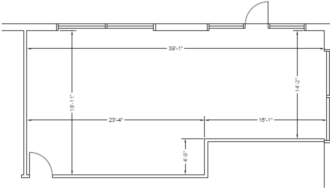
1275 12th Ave NW (07-09-07) - Floor 01
